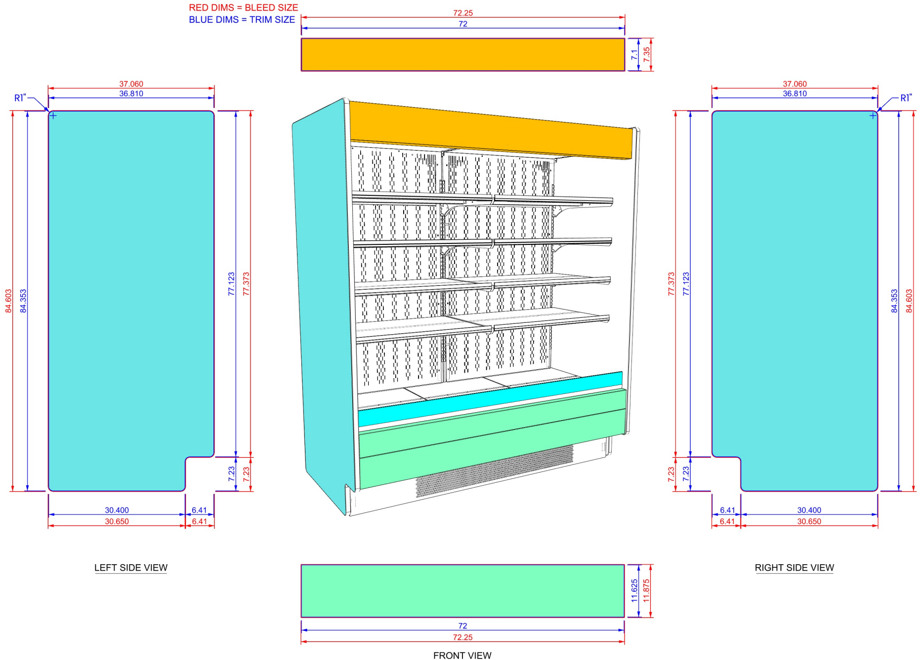
FRONT VIEW
