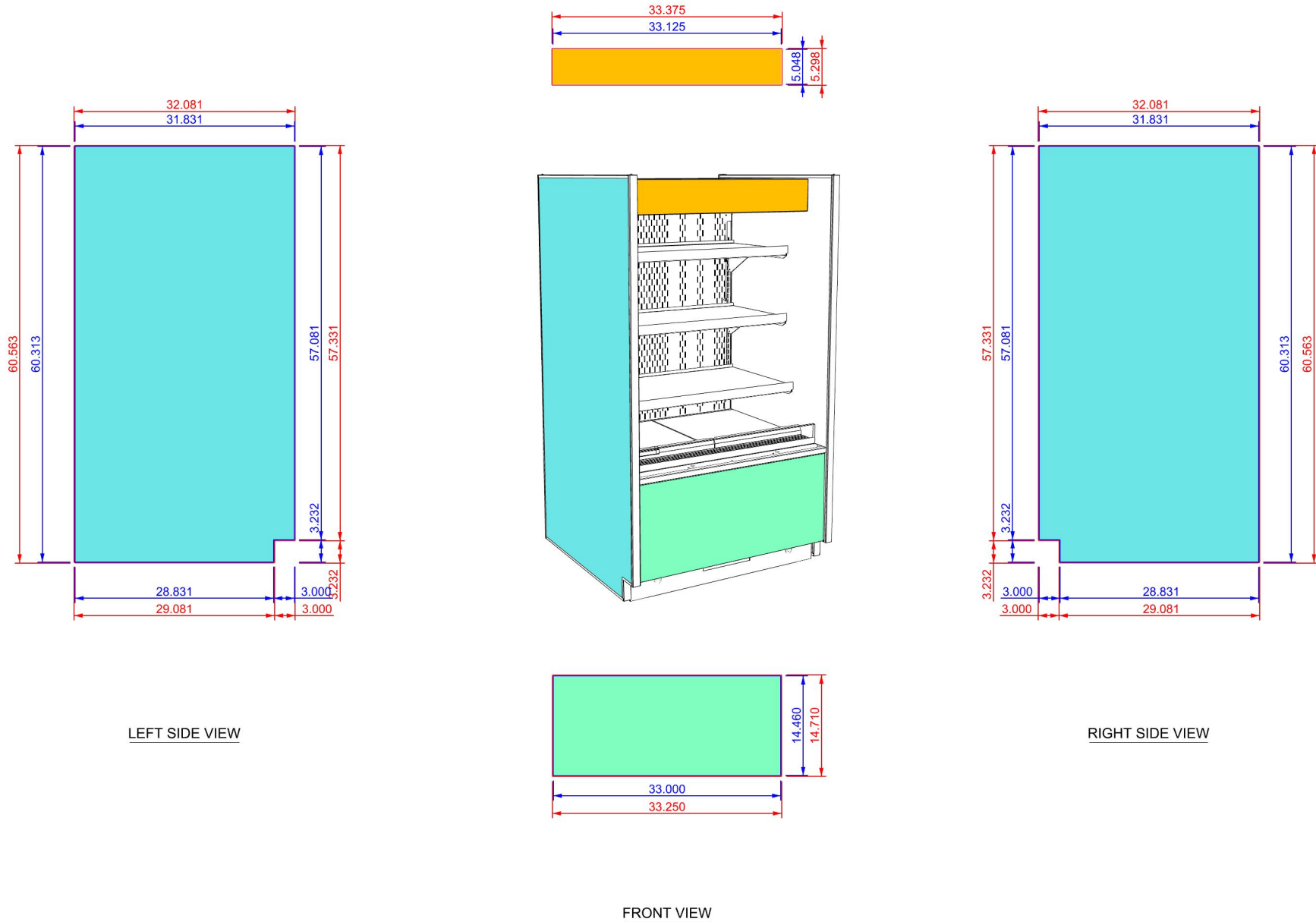
FRONT VIEW
