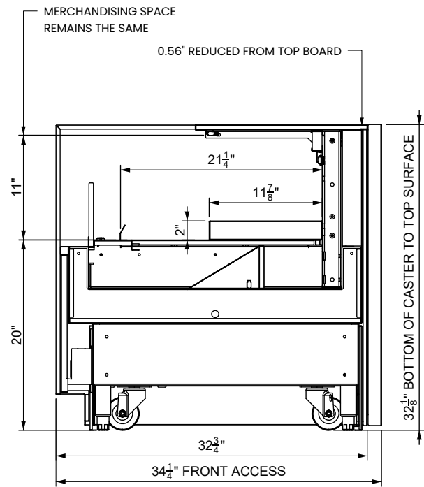
REDUCED HEIGHT MODEL
