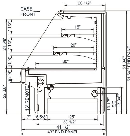
FLAT ANGLED OPTION PROFILE
