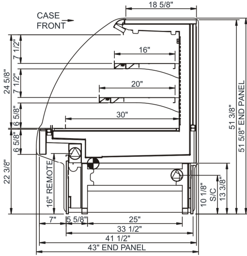
STANDARD CURVED PROFILE
